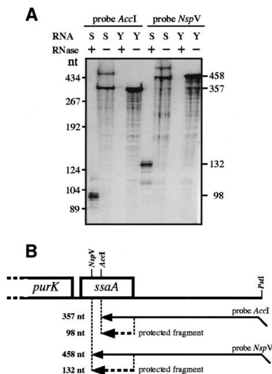
Fig. 3. Ribonuclease protection assay. A: Synthesized RNA probes from plasmid pPPI.5 linearized by AccI or NspV were incubated with Synechococcus PCC6301 RNA (lanes S) or yeast total RNA (lanes Y) followed by digestion with (lanes +) or without (lanes −) RNases A and T 1 . DNA molecular markers are HaeIII digests of pBR322. B: The experimental design of the ribonuclease protection assays is shown. Solid arrows indicate RNA probes (458 nt, 357 nt) and dashed arrows indicate protected products.
