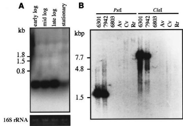
Fig. 5. A: Northern analysis of Synechococcus PCC6301 6Sa RNA. RNAs were isolated from cells of early-log phase, mid-log phase, late-log phase and stationary phase. B: Southern analysis by cross-hybridization of Synechococcus PCC6301 6Sa RNA gene. Genomic DNAs were prepared from Synechococcus PCC6301 (6301), Synechococcus PCC7942 (7942), Synechocystis PCC6803 (6803), A. variabilis (Av), C. vinosum (Cv) and R. rubrum (Rr) and digested with Pst I or Cl aI.
